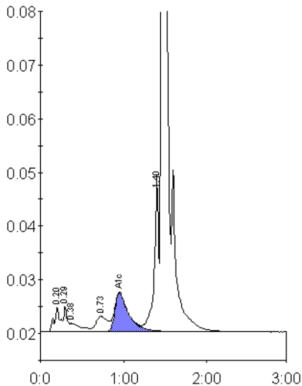
Peak table - ID: 10488234
